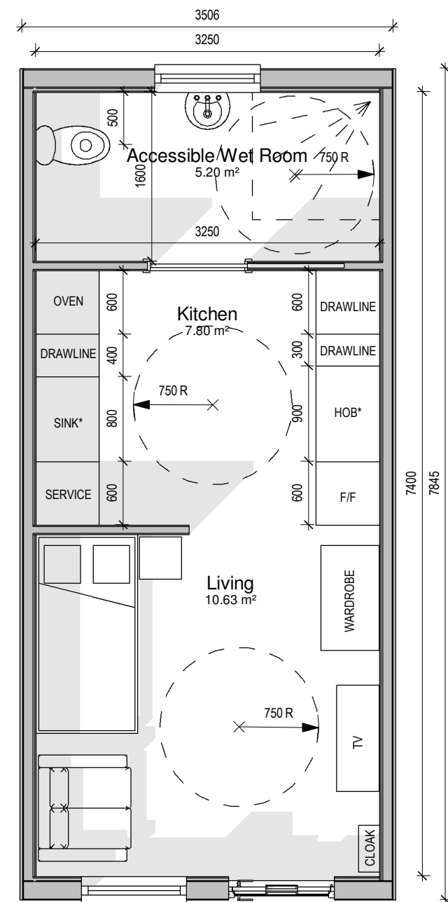
Unit Type - Accessible Single GIA - 24.05m 2 Arrangement - Centre
