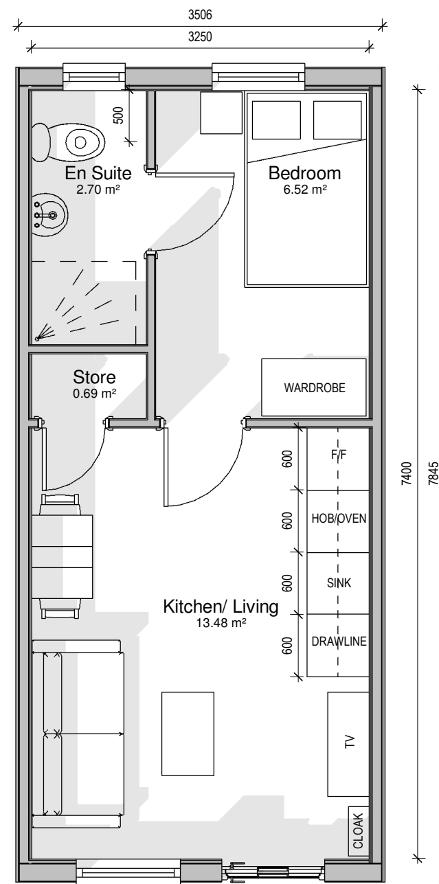
Unit Type - Standard Single/ Double GIA - 24.05m 2 Arrangement - Centre
