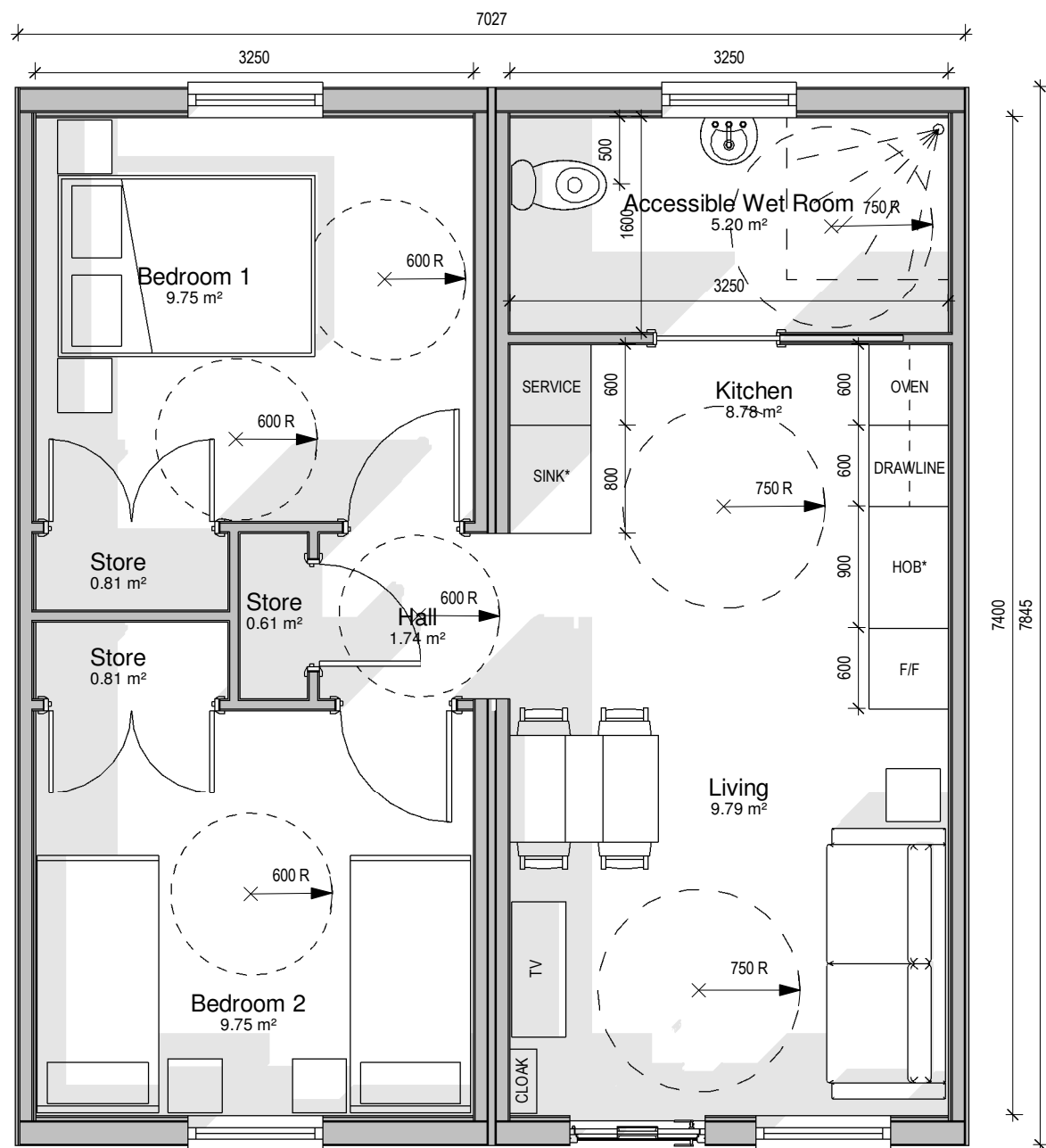
Unit Type - Accessible Family GIA - 50.11m 2 Arrangement - Centre
